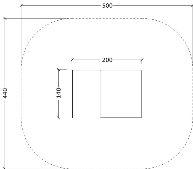
Plan, safety zone
