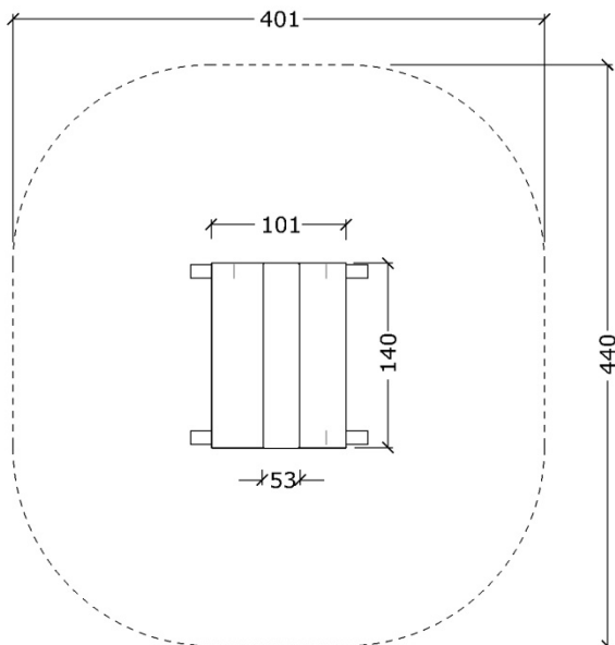
Plan, safety zone
